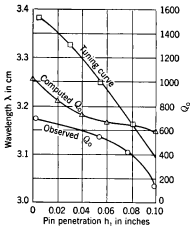
FIG. 14.5.—Cold-resonance data for the sprocket-tunable magnetron. h_0 = 0.250 in.; d_0 = 0.086 in.; d_1 = 0.0623 in.; \delta/\lambda = 2.1 \times 10^{-6} for copper at 3.2 cm; Q_0 was computed from Eq. (11.10).
